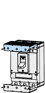
Assembly Diagram
